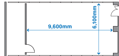
Floor plan
